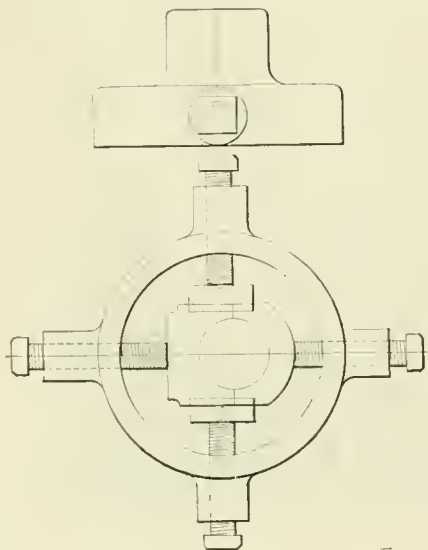
CHUCKING ROD BRASSES.
